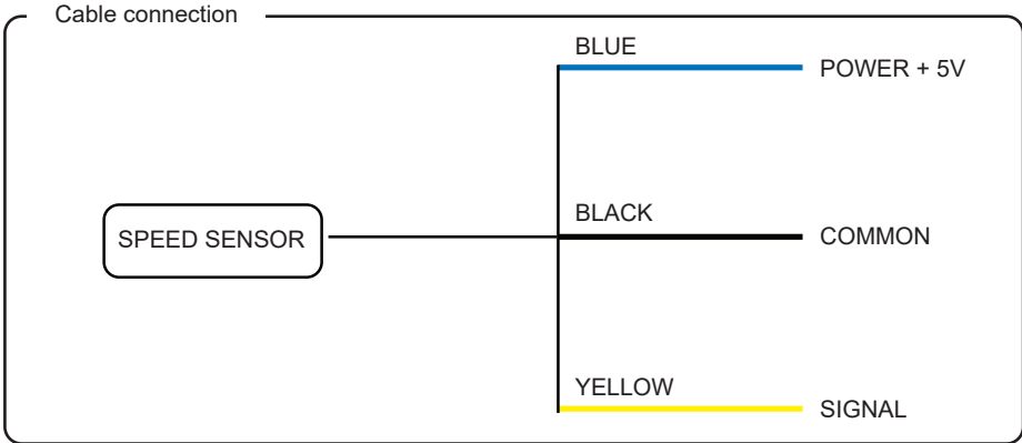
YST BB993 Speed sensor signal - VOLT Sheet
